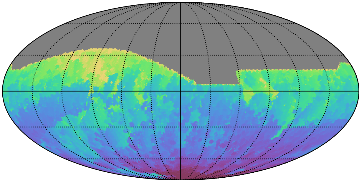
too_elab_heavy_r32_d3_griz_v3.4_10yrs All sky i band: Min HA
