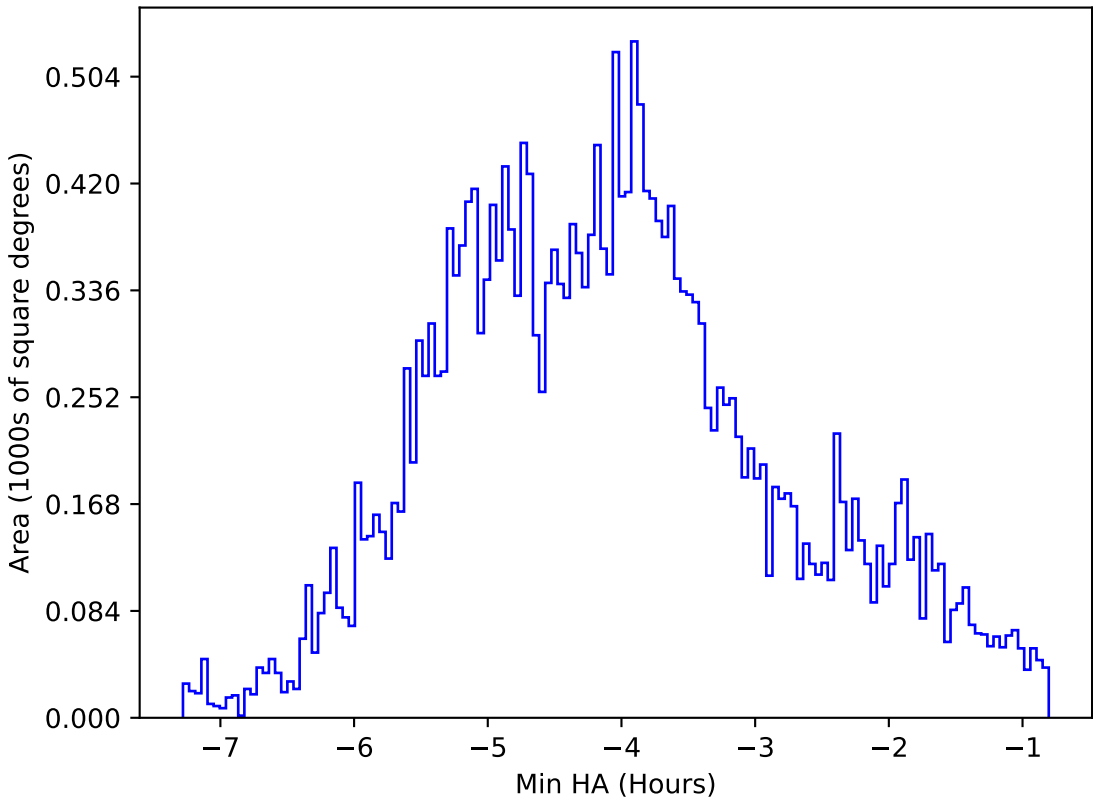
too_elab_heavy_r32_d3_griz_v3.4_10yrs All sky i band: Min HA
