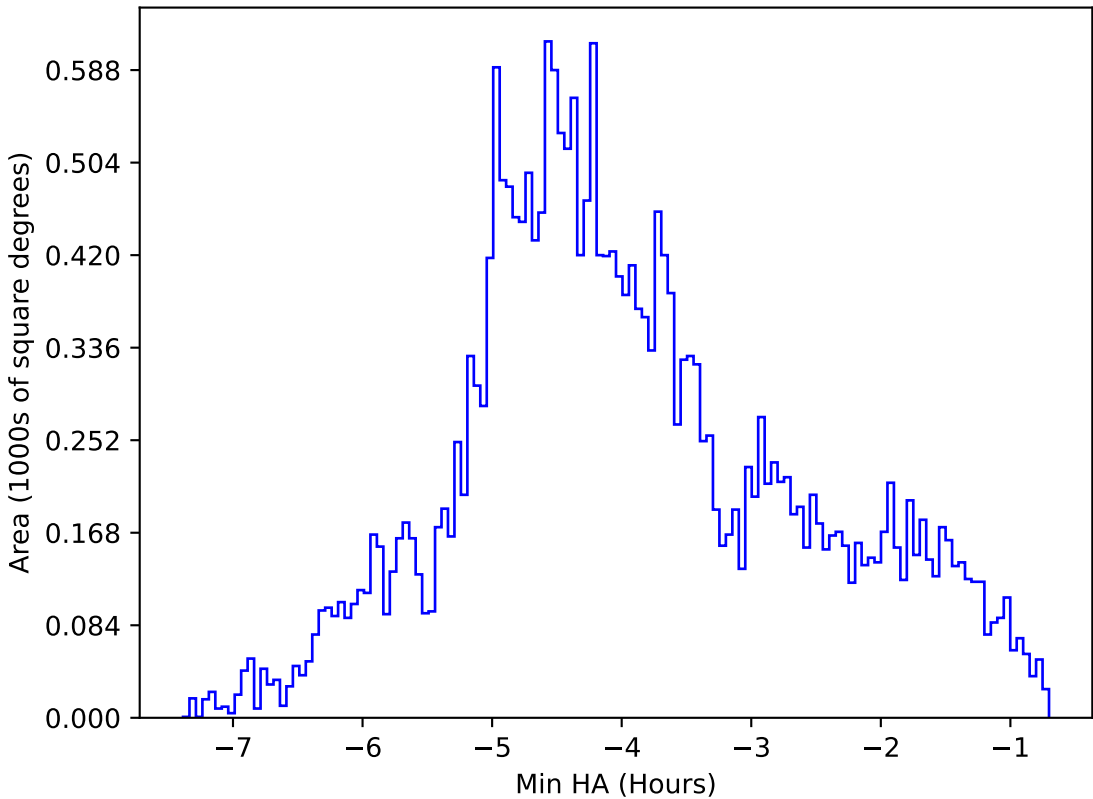
too_elab_heavy_r32_d3_griz_v3.4_10yrs All sky g band: Min HA
