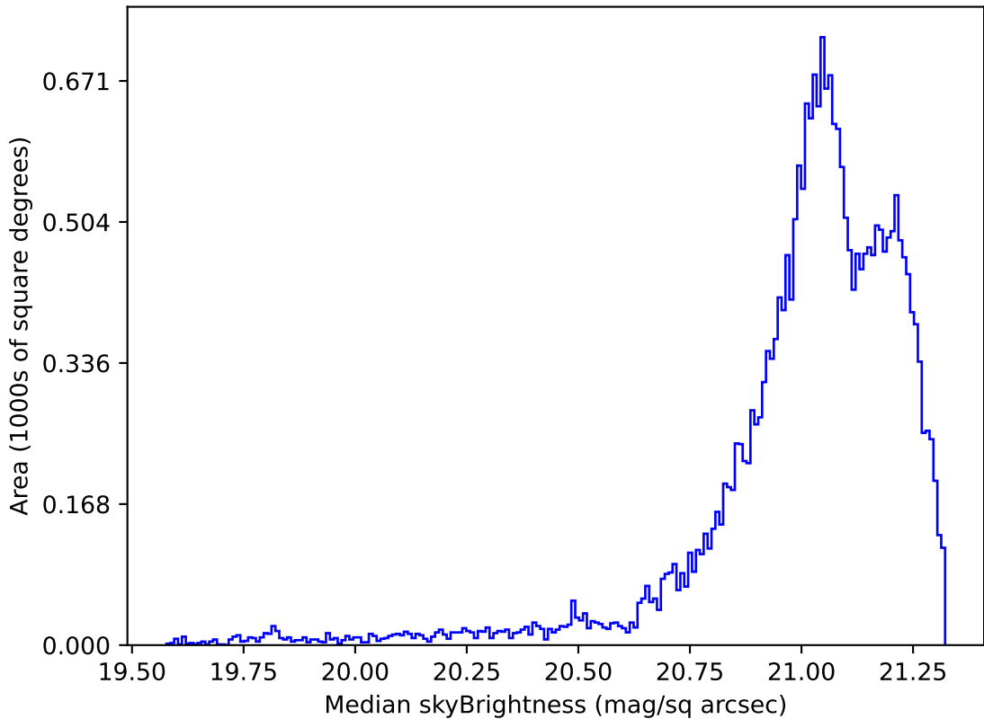
too_elab_heavy_r32_d3_griz_v3.4_10yrs Yr 1 r band: Median skyBrightness
