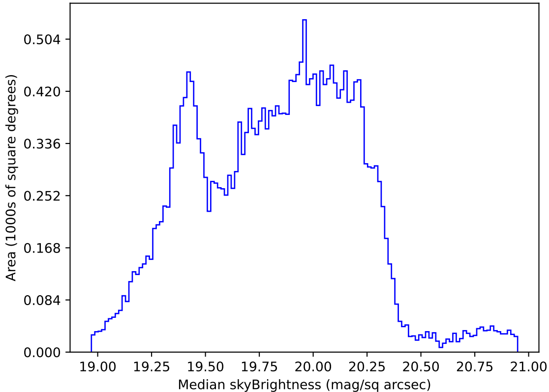
too_elab_heavy_r32_d3_griz_v3.4_10yrs Yr 1 all bands: Median skyBrightness
