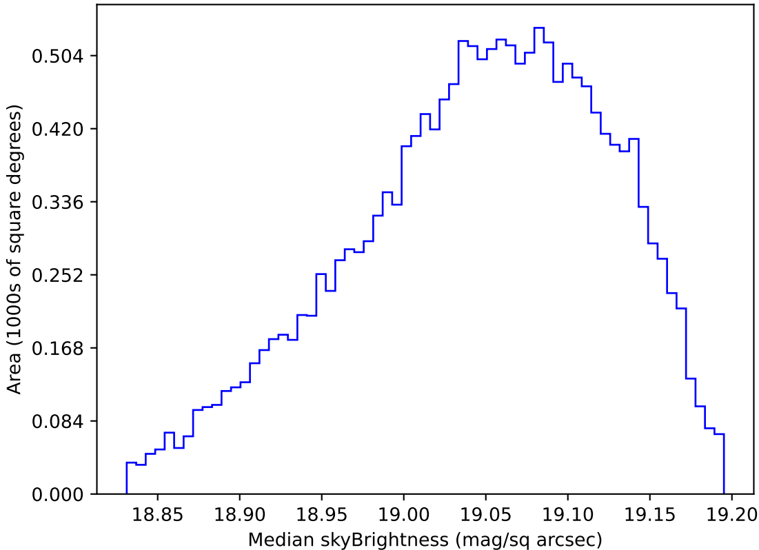
too_elab_heavy_r32_d3_griz_v3.4_10yrs WFD z band: Median skyBrightness
