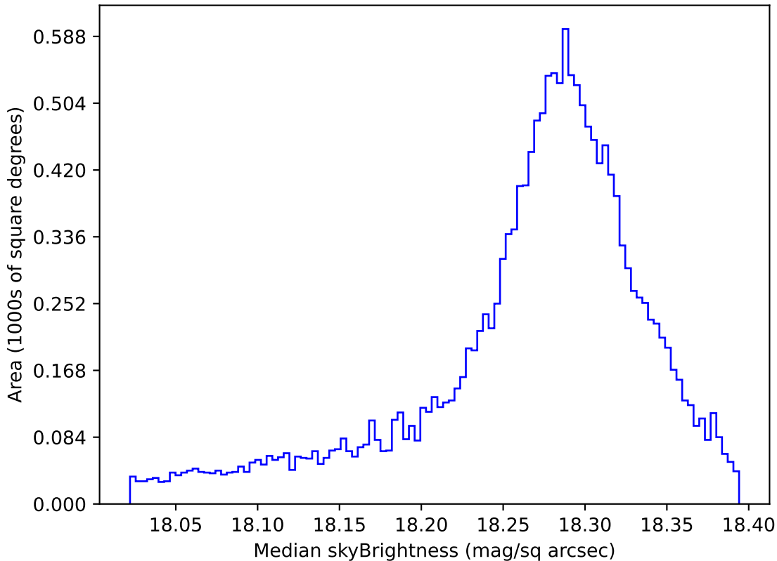
too_elab_heavy_r32_d3_griz_v3.4_10yrs WFD y band: Median skyBrightness
