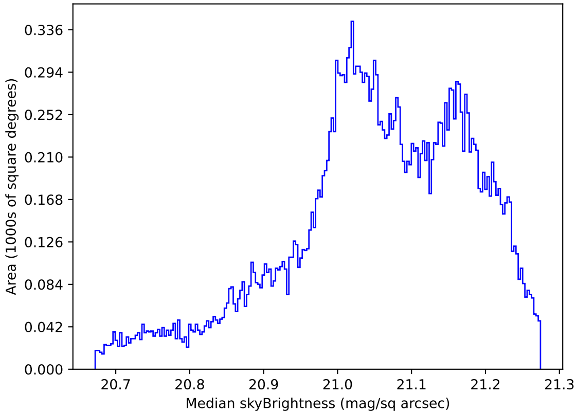
too_elab_heavy_r32_d3_griz_v3.4_10yrs All sky r band: Median skyBrightness
