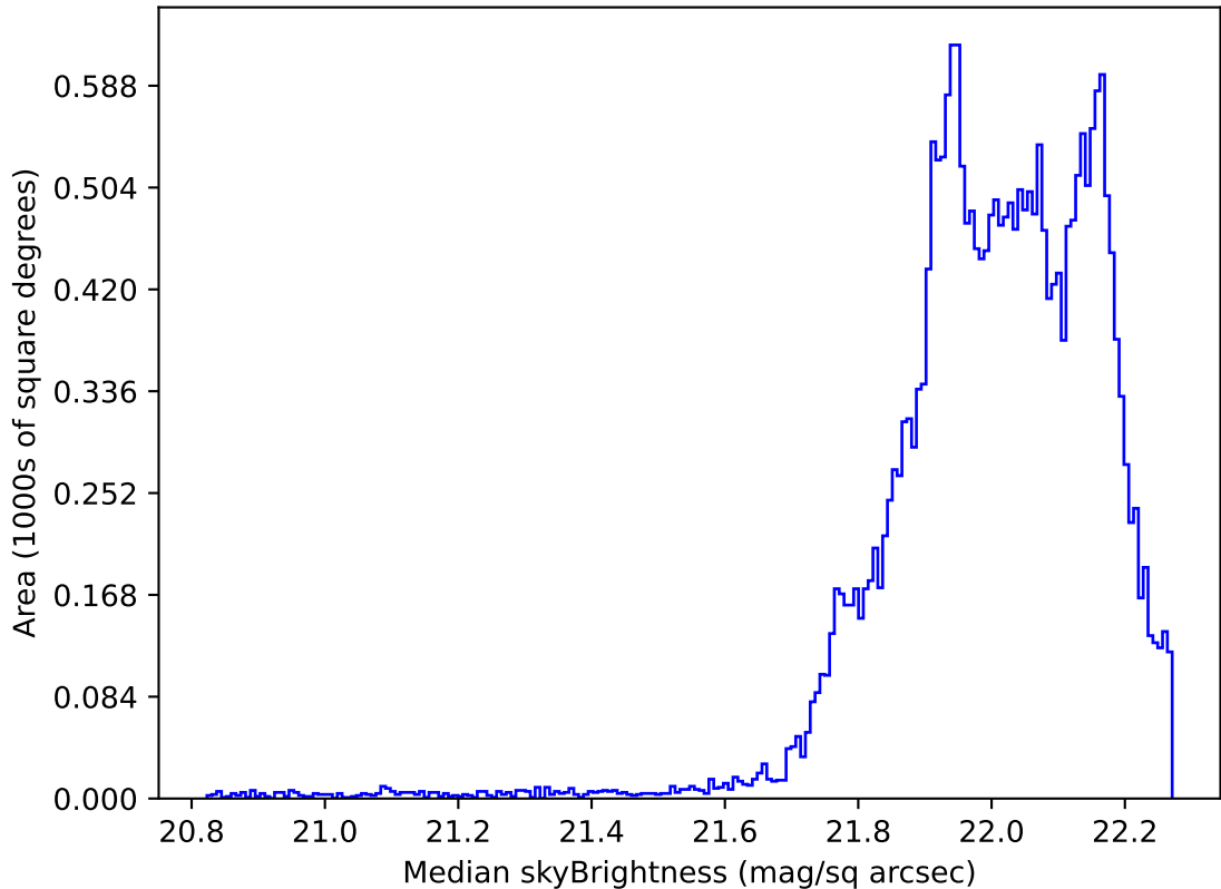
too_elab_heavy_r32_d3_griz_v3.4_10yrs All sky g band: Median skyBrightness
