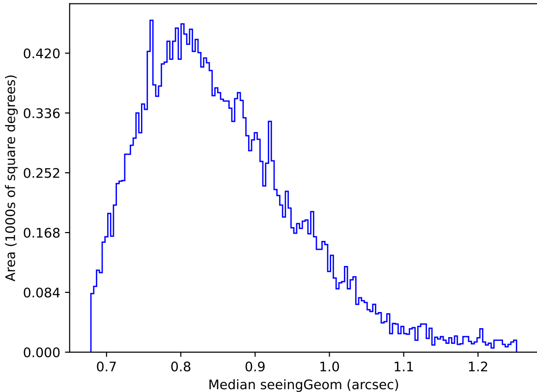
too_elab_heavy_r32_d3_griz_v3.4_10yrs Yr 1 z band: Median seeingGeom
