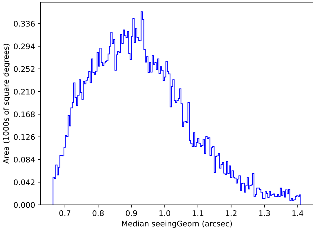
too_elab_heavy_r32_d3_griz_v3.4_10yrs Yr 1 g band: Median seeingGeom
