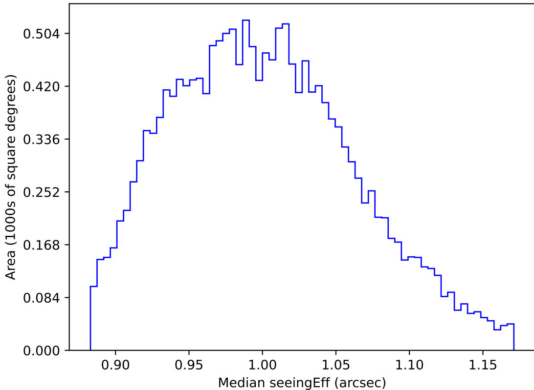
too_elab_heavy_r32_d3_griz_v3.4_10yrs WFD y band: Median seeingEff
