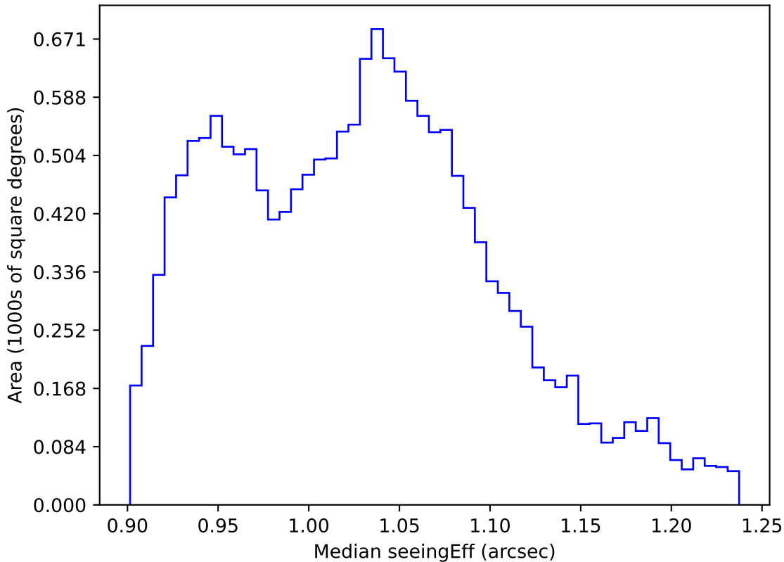
too_elab_heavy_r32_d3_griz_v3.4_10yrs WFD all bands: Median seeingEff
