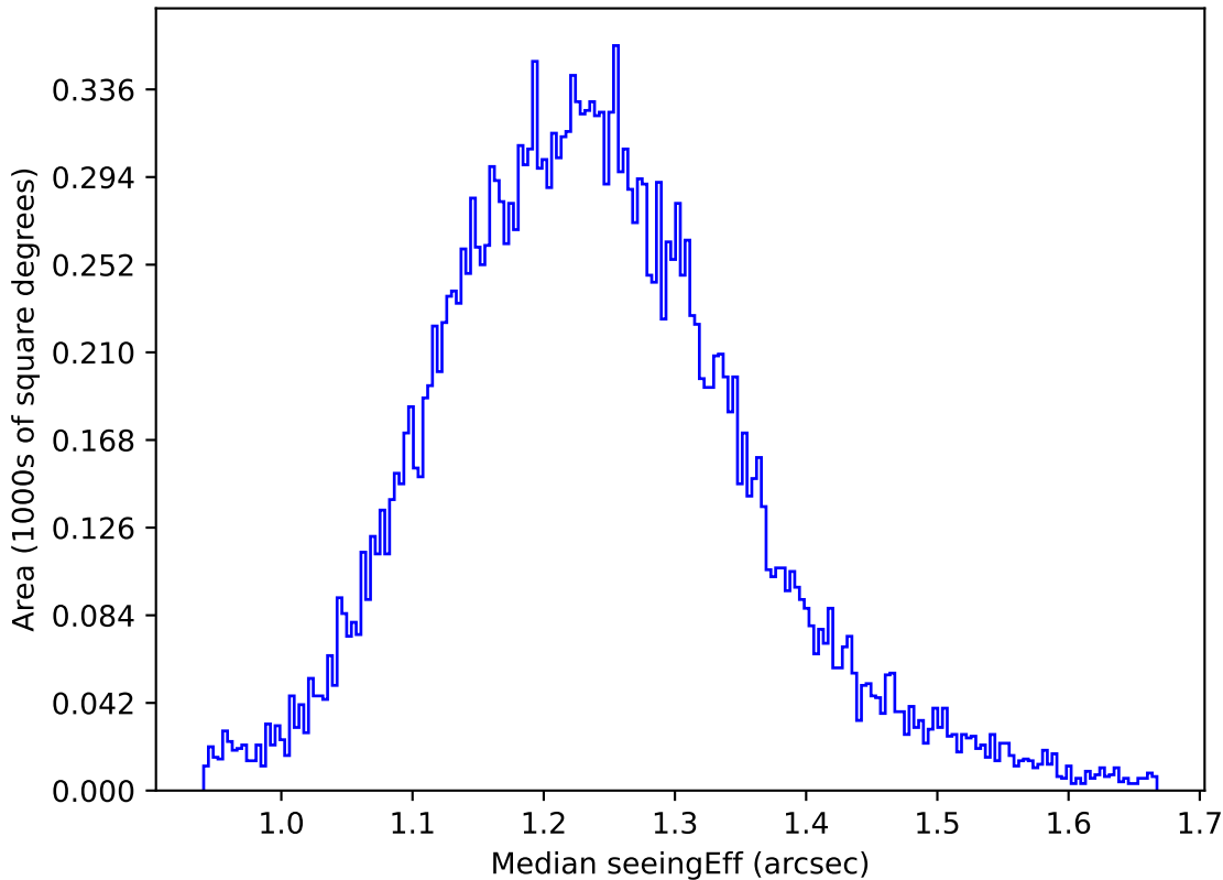
too_elab_heavy_r32_d3_griz_v3.4_10yrs All sky u band: Median seeingEff
