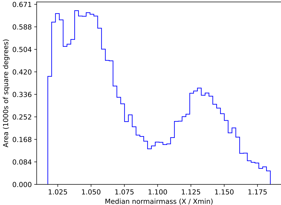
too_elab_heavy_r32_d3_griz_v3.4_10yrs WFD r band: Median normairmass
