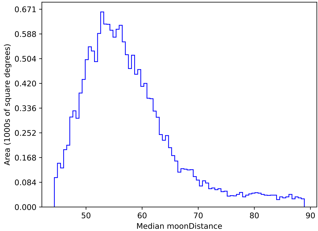
too_elab_heavy_r32_d3_griz_v3.4_10yrs WFD y band: Median moonDistance
