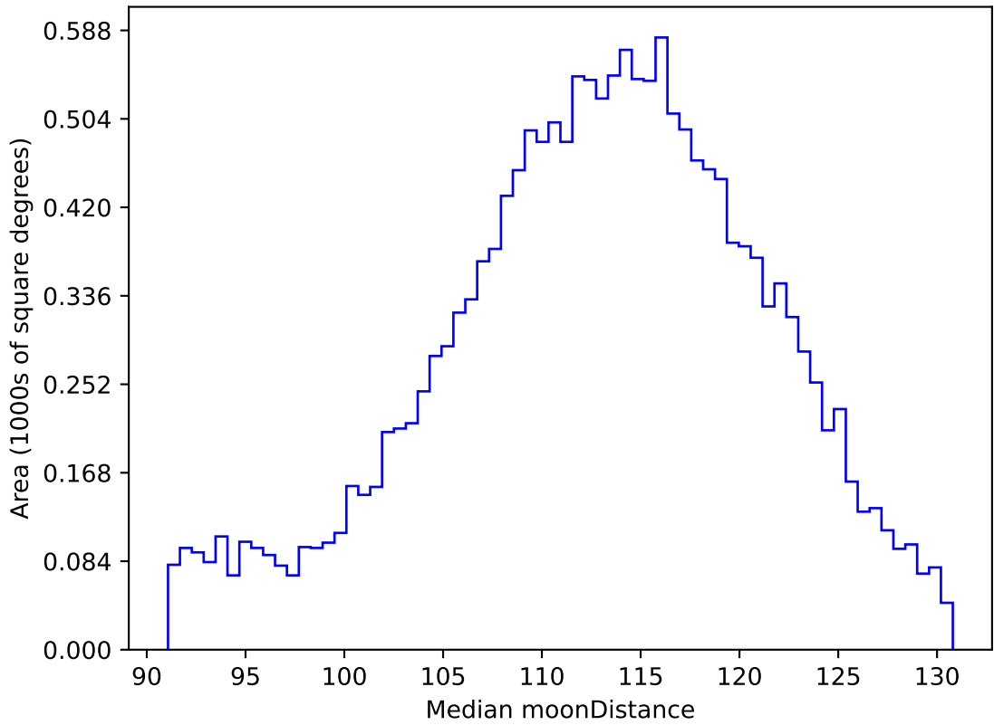
too_elab_heavy_r32_d3_griz_v3.4_10yrs WFD r band: Median moonDistance
