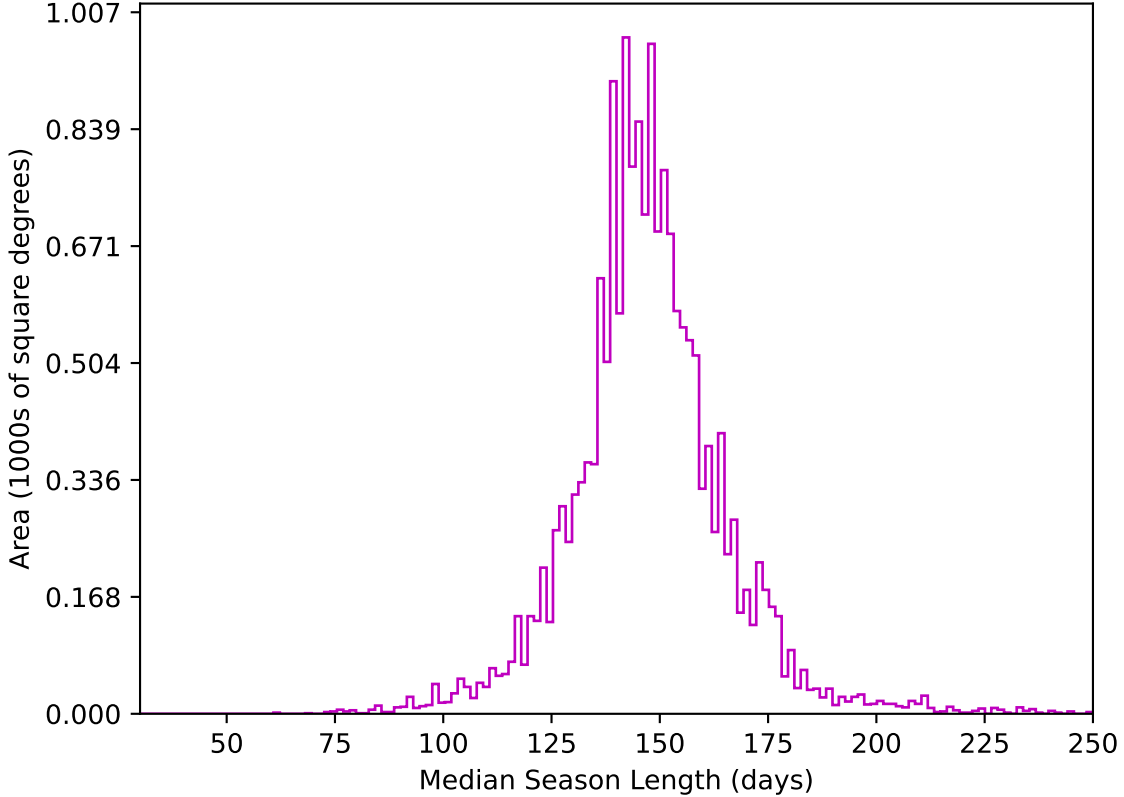
too_elab_heavy_r32_d3_griz_v3.4_10yrs WFD z band: Median Season Length
