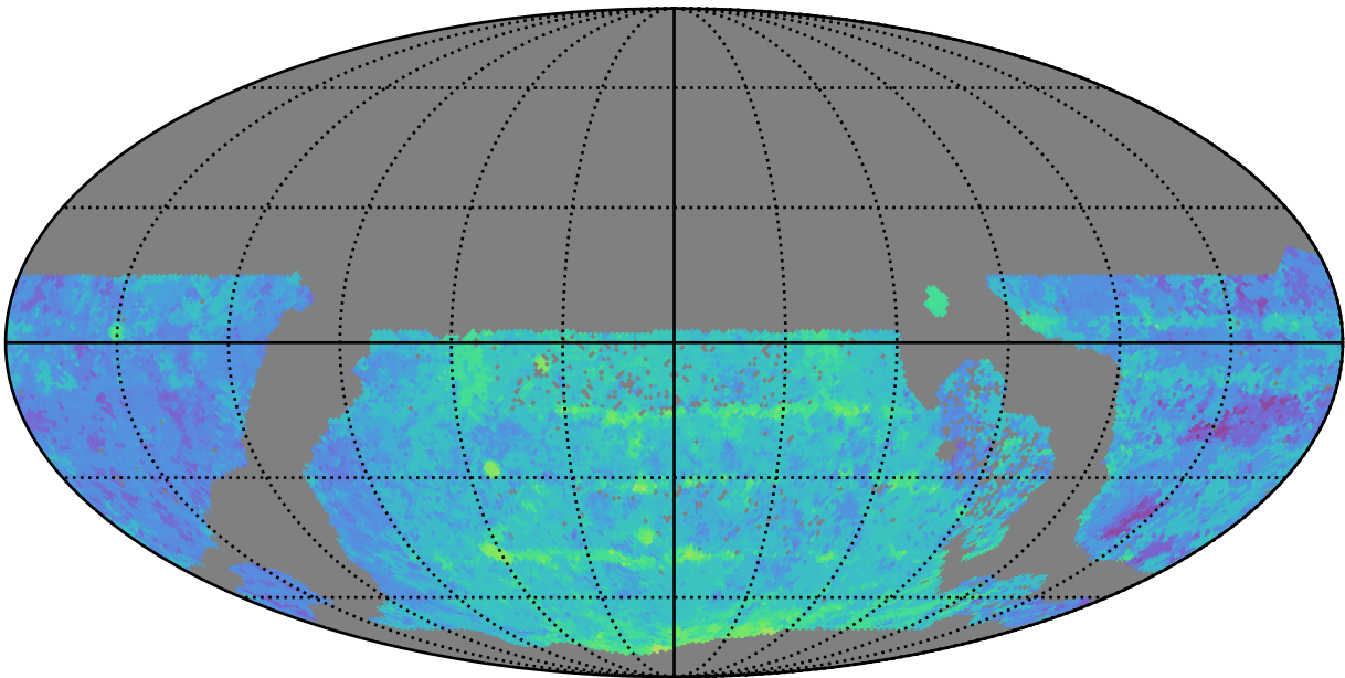
too_elab_heavy_r32_d3_griz_v3.4_10yrs WFD y band: Median Season Length
