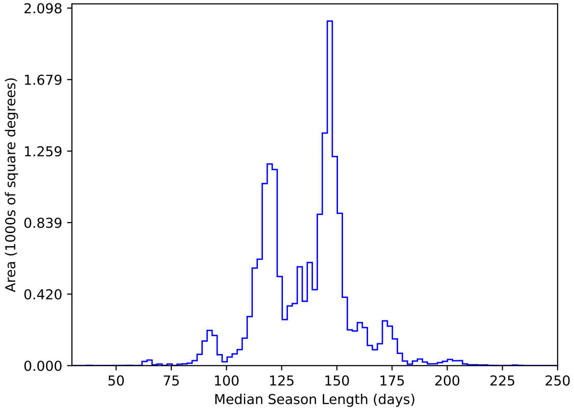
too_elab_heavy_r32_d3_griz_v3.4_10yrs WFD y band: Median Season Length
