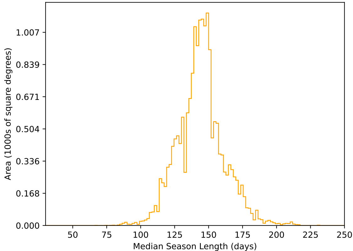
too_elab_heavy_r32_d3_griz_v3.4_10yrs WFD r band: Median Season Length
