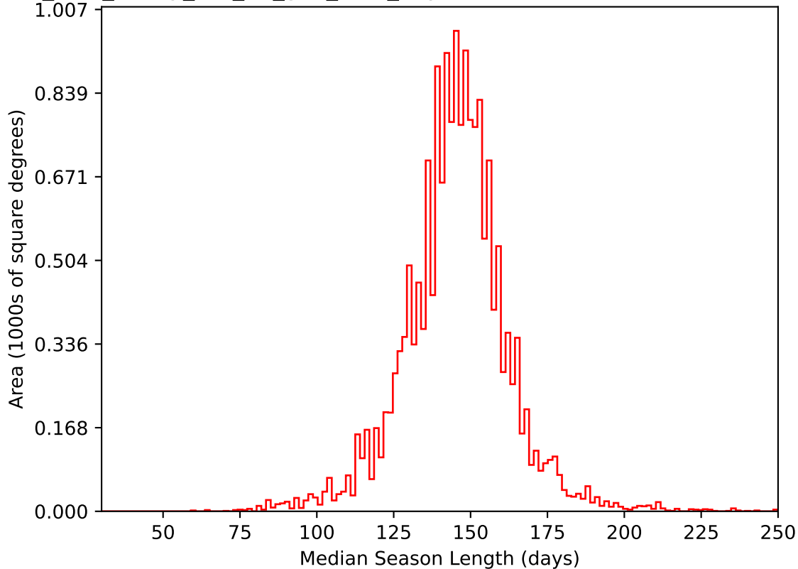
too_elab_heavy_r32_d3_griz_v3.4_10yrs WFD i band: Median Season Length
