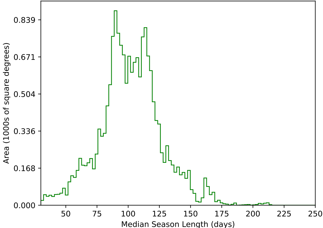
too_elab_heavy_r32_d3_griz_v3.4_10yrs WFD g band: Median Season Length
