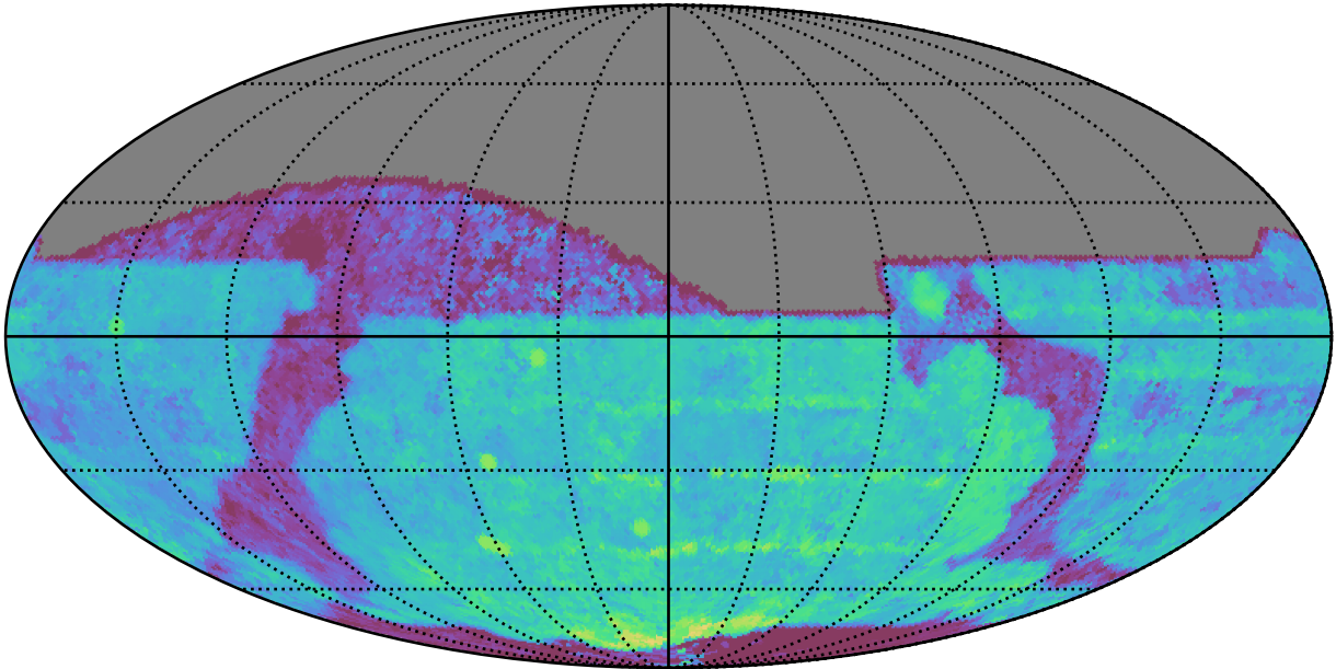
too_elab_heavy_r32_d3_griz_v3.4_10yrs All sky z band: Median Season Length
