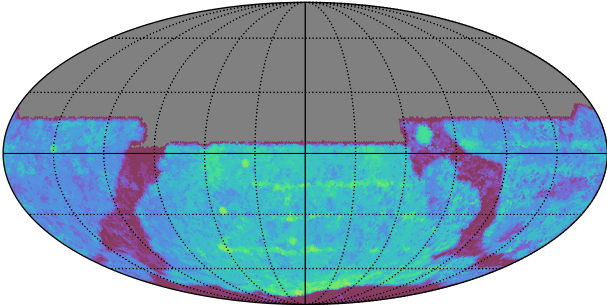
too_elab_heavy_r32_d3_griz_v3.4_10yrs All sky y band: Median Season Length
