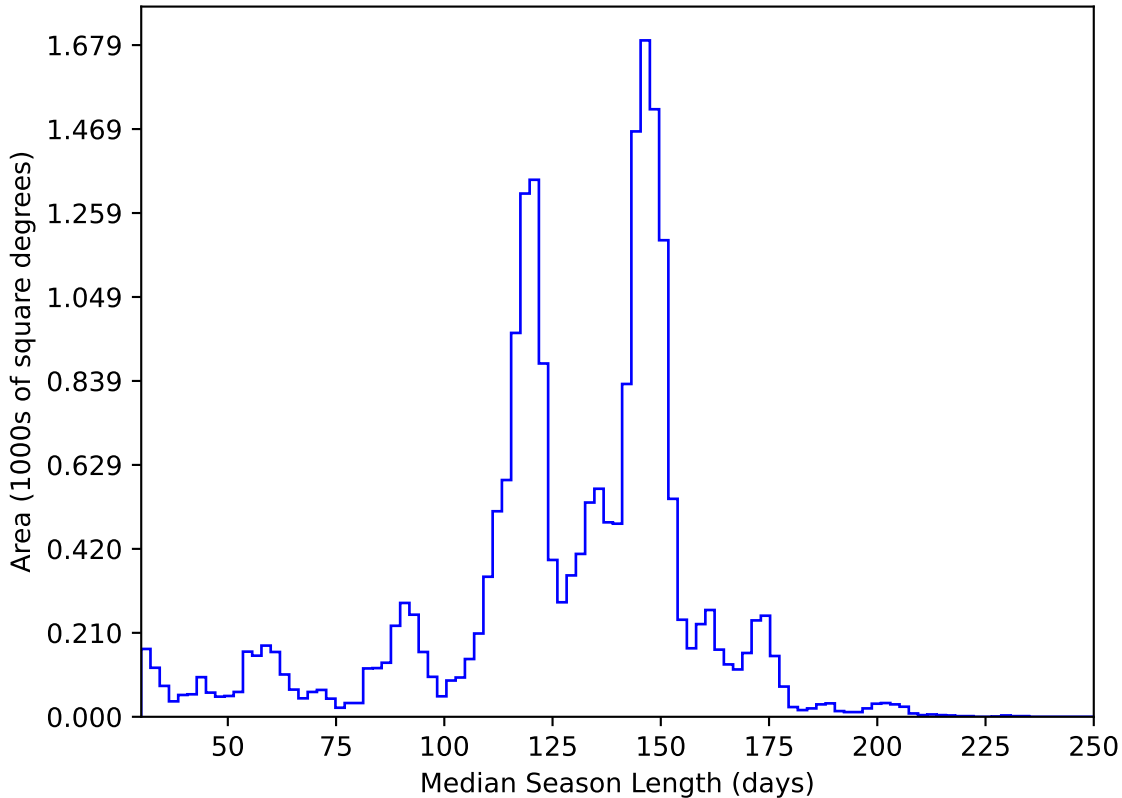
too_elab_heavy_r32_d3_griz_v3.4_10yrs All sky y band: Median Season Length
