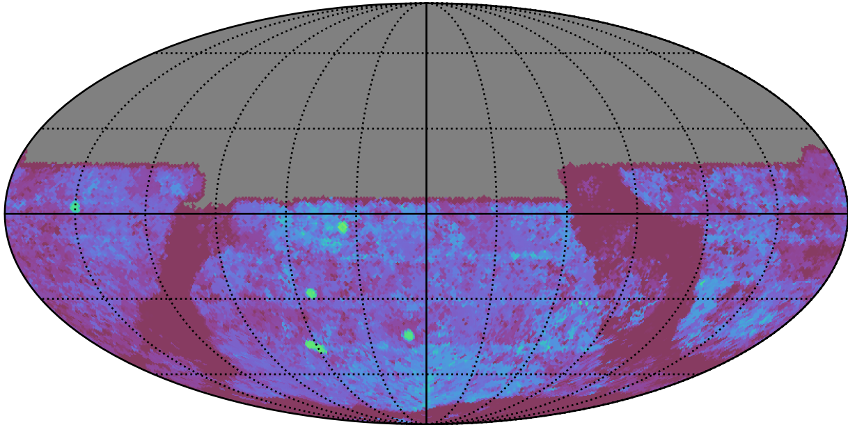
too_elab_heavy_r32_d3_griz_v3.4_10yrs All sky u band: Median Season Length
