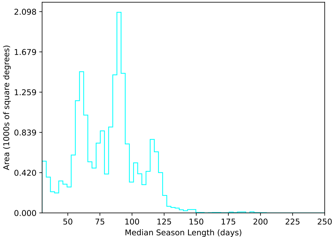
too_elab_heavy_r32_d3_griz_v3.4_10yrs All sky u band: Median Season Length
