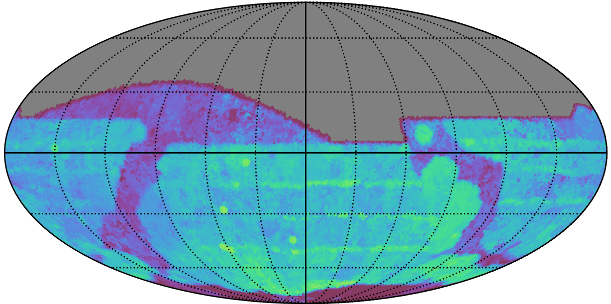
too_elab_heavy_r32_d3_griz_v3.4_10yrs All sky r band: Median Season Length
