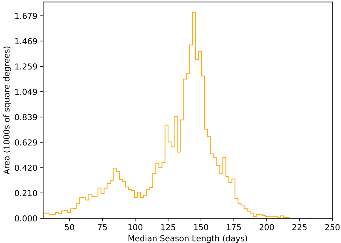
too_elab_heavy_r32_d3_griz_v3.4_10yrs All sky r band: Median Season Length
