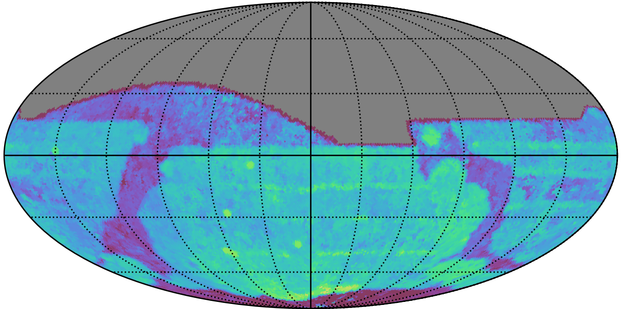
too_elab_heavy_r32_d3_griz_v3.4_10yrs All sky i band: Median Season Length
