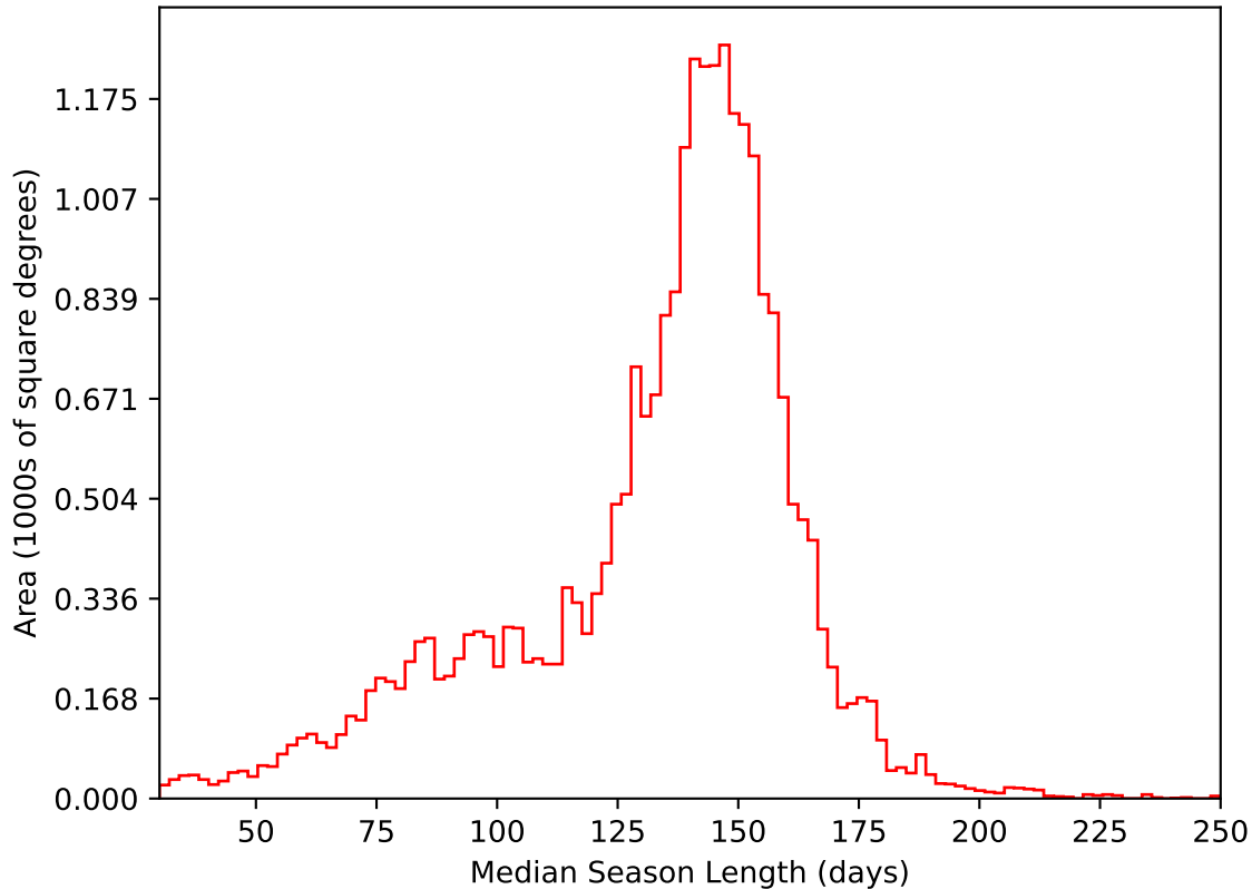
too_elab_heavy_r32_d3_griz_v3.4_10yrs All sky i band: Median Season Length
