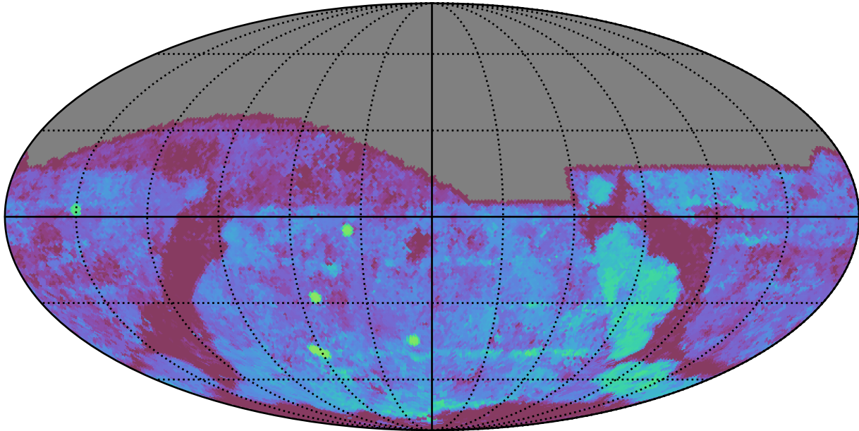
too_elab_heavy_r32_d3_griz_v3.4_10yrs All sky g band: Median Season Length
