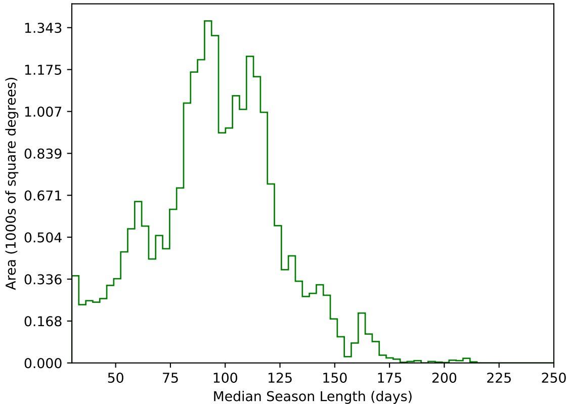
too_elab_heavy_r32_d3_griz_v3.4_10yrs All sky g band: Median Season Length
