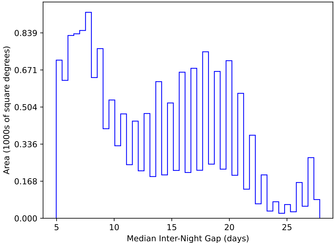
too_elab_heavy_r32_d3_griz_v3.4_10yrs WFD y band: Median Inter-Night Gap
