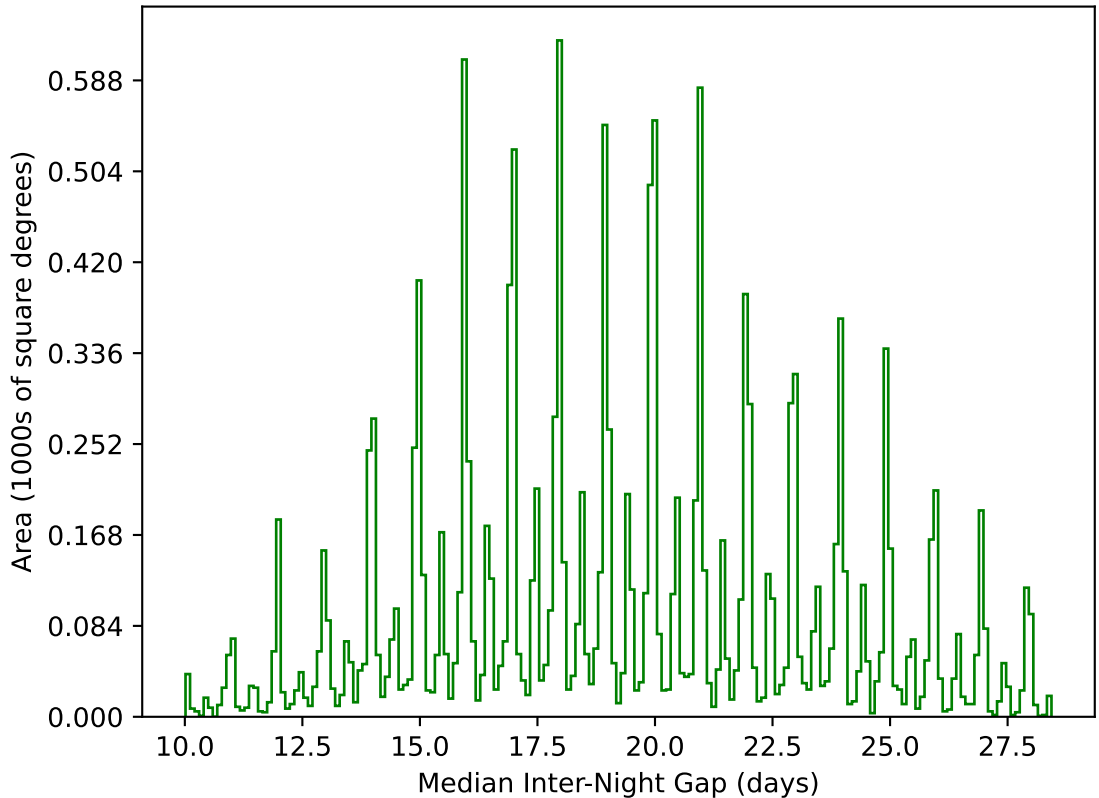
too_elab_heavy_r32_d3_griz_v3.4_10yrs WFD g band: Median Inter-Night Gap
