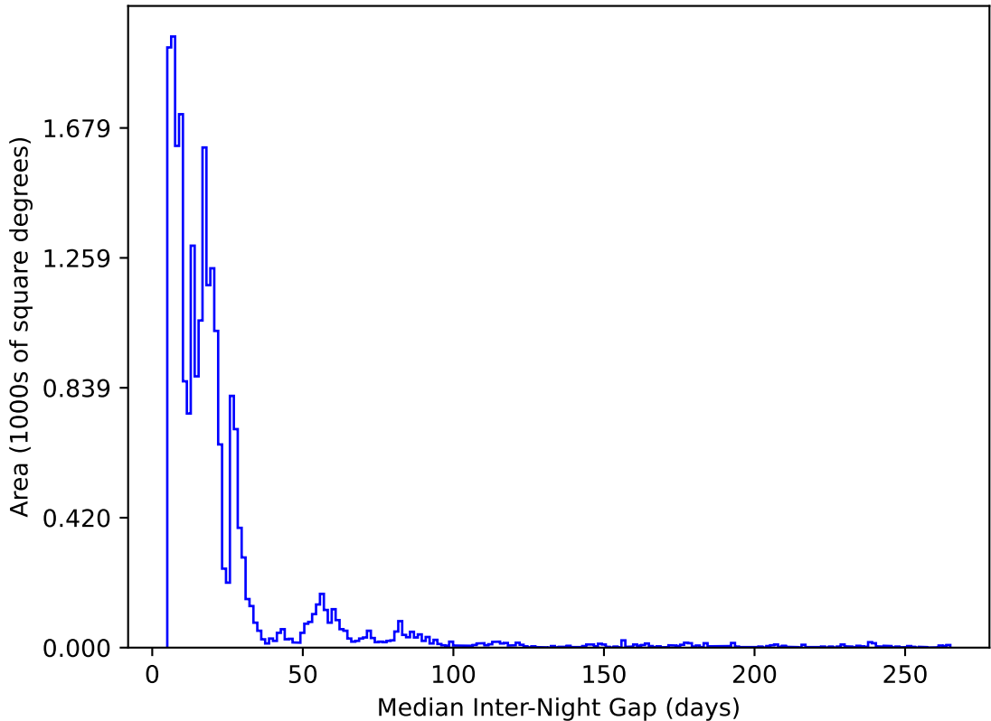
too_elab_heavy_r32_d3_griz_v3.4_10yrs All sky y band: Median Inter-Night Gap
