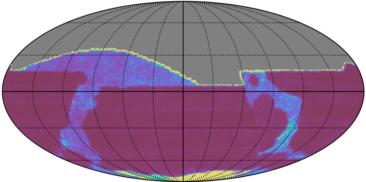
too_elab_heavy_r32_d3_griz_v3.4_10yrs All sky r band: Median Inter-Night Gap
