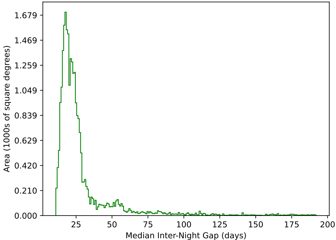
too_elab_heavy_r32_d3_griz_v3.4_10yrs All sky g band: Median Inter-Night Gap
