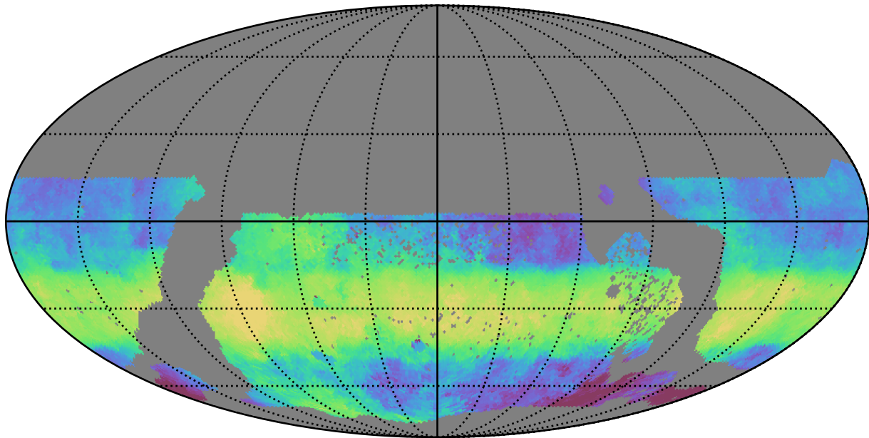
too_elab_heavy_r32_d3_griz_v3.4_10yrs WFD z band: Median HA
