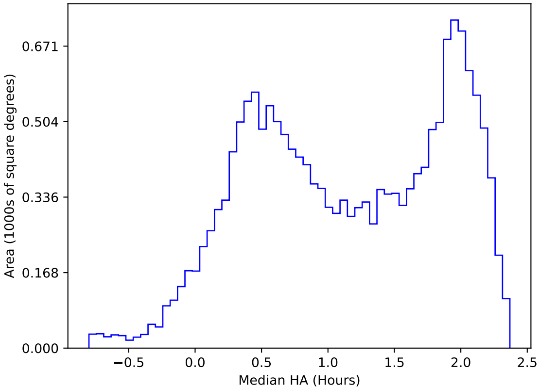
too_elab_heavy_r32_d3_griz_v3.4_10yrs WFD z band: Median HA
