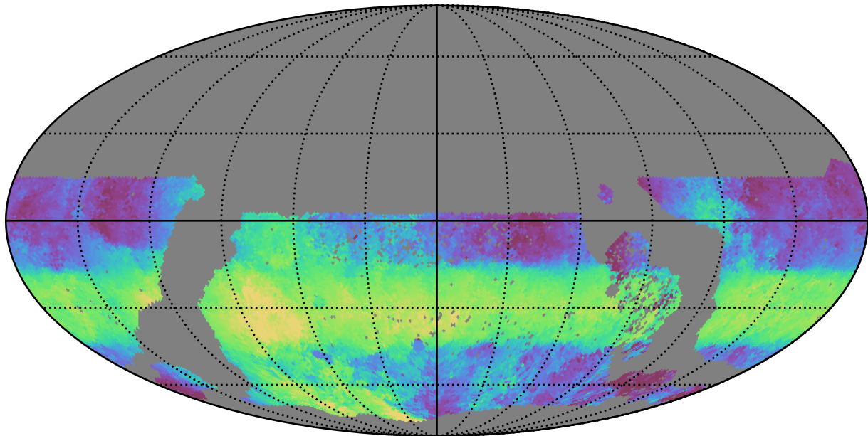
too_elab_heavy_r32_d3_griz_v3.4_10yrs WFD u band: Median HA
