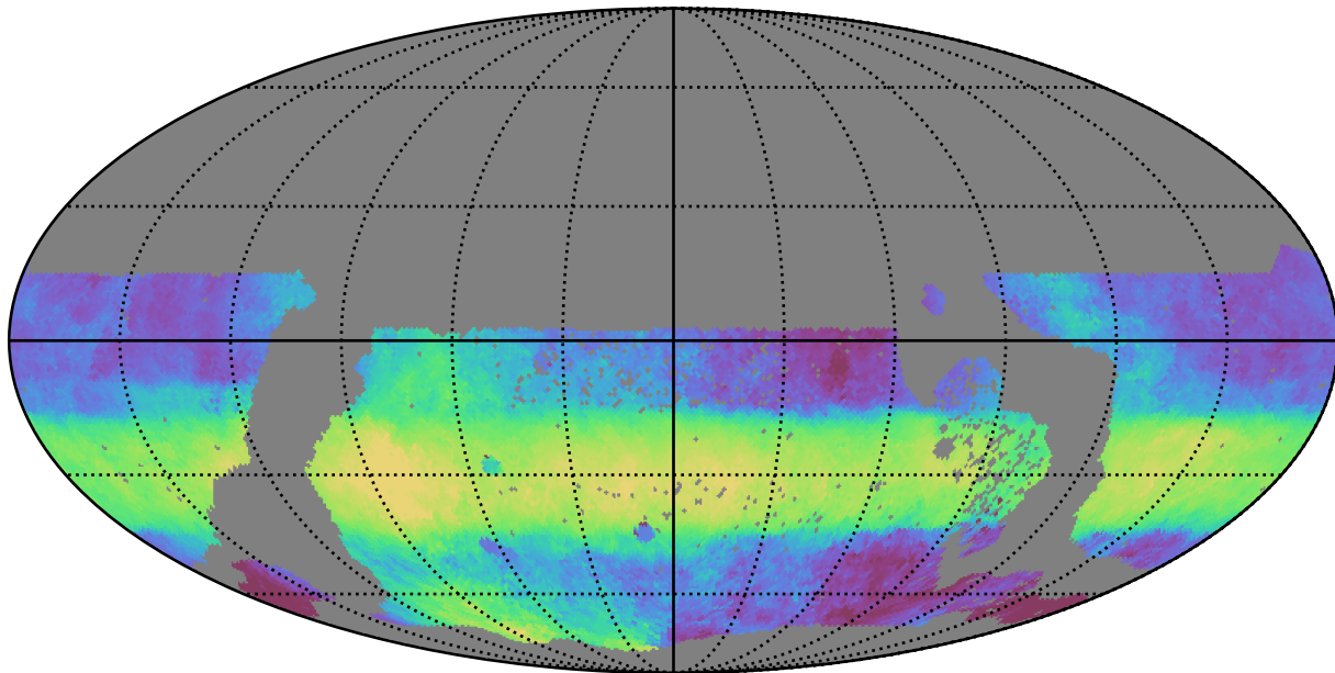
too_elab_heavy_r32_d3_griz_v3.4_10yrs WFD r band: Median HA
