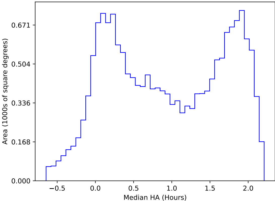
too_elab_heavy_r32_d3_griz_v3.4_10yrs WFD r band: Median HA
