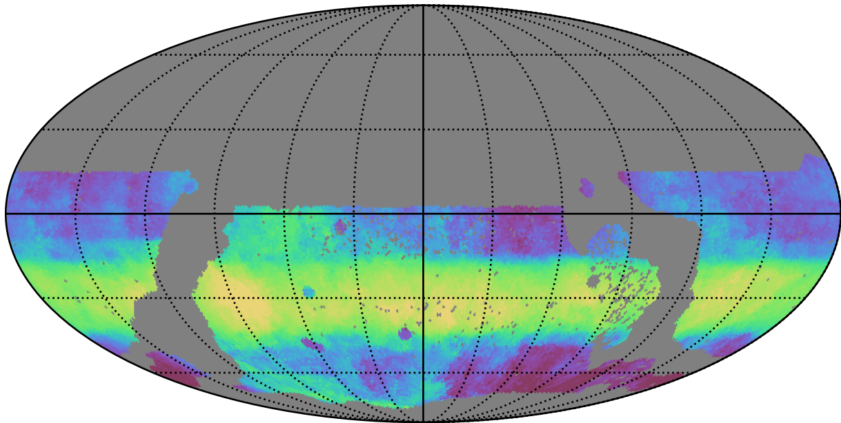
too_elab_heavy_r32_d3_griz_v3.4_10yrs WFD i band: Median HA
