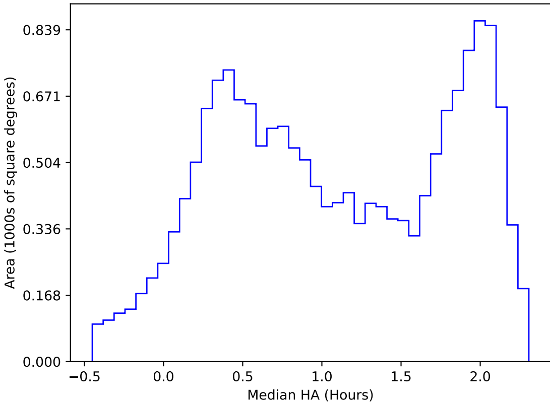
too_elab_heavy_r32_d3_griz_v3.4_10yrs WFD i band: Median HA
