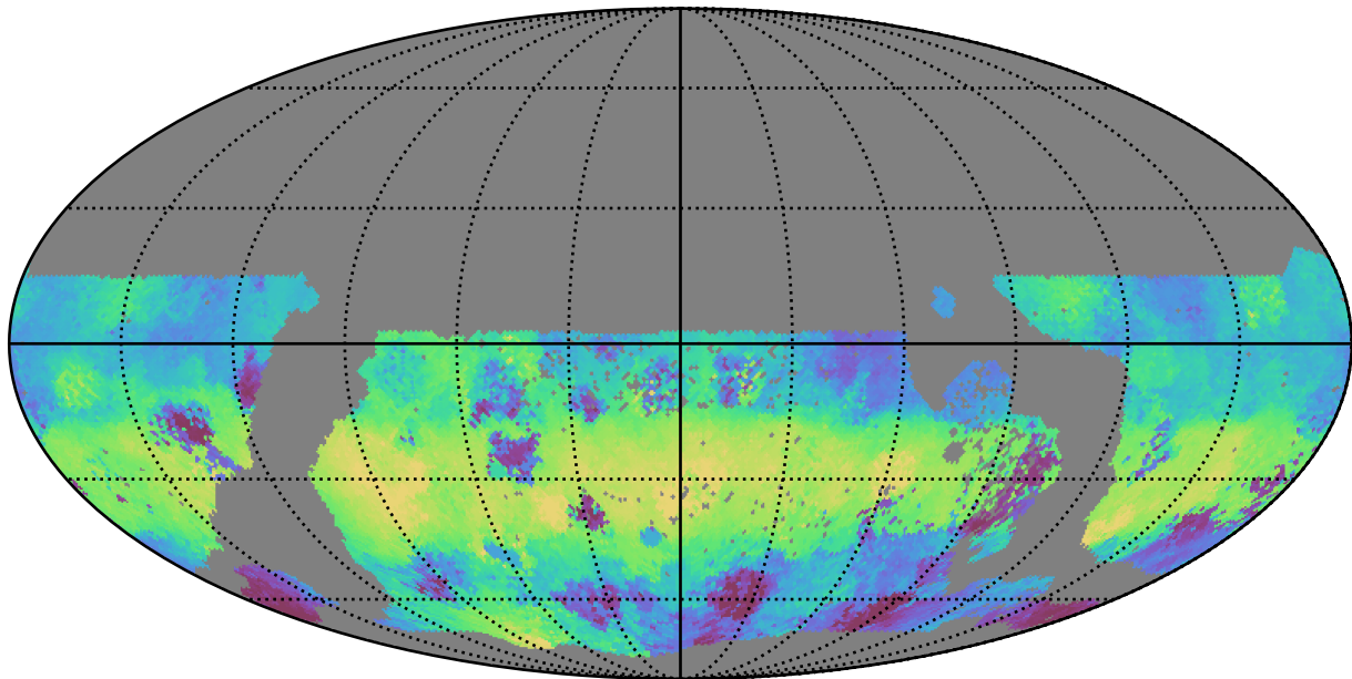
too_elab_heavy_r32_d3_griz_v3.4_10yrs WFD g band: Median HA
