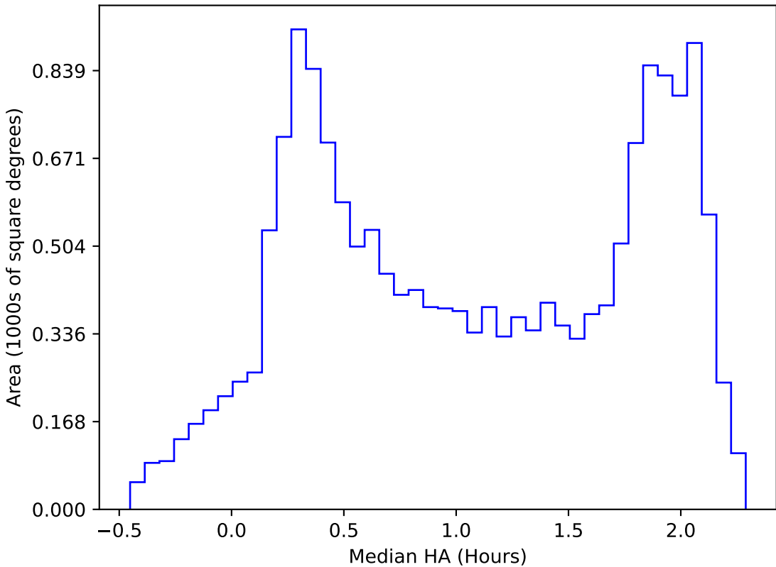
too_elab_heavy_r32_d3_griz_v3.4_10yrs WFD all bands: Median HA
