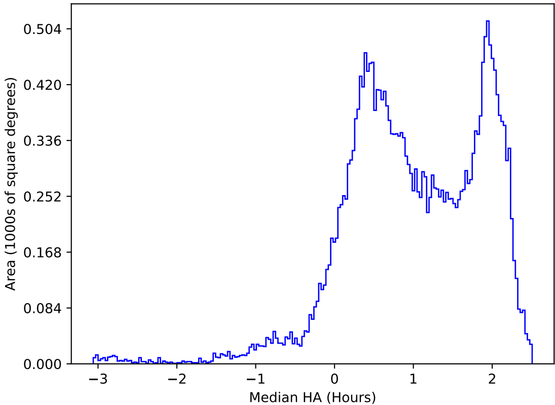
too_elab_heavy_r32_d3_griz_v3.4_10yrs All sky z band: Median HA
