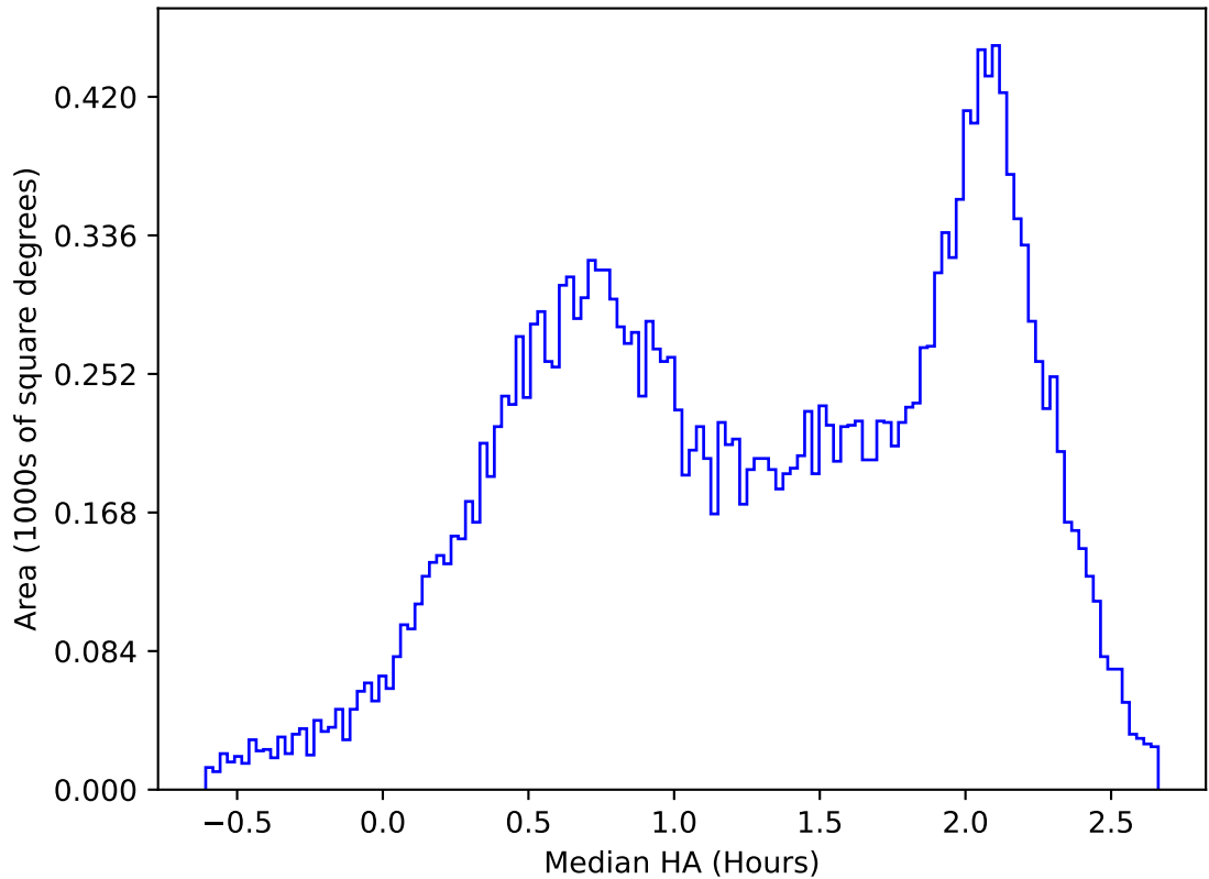
too_elab_heavy_r32_d3_griz_v3.4_10yrs All sky y band: Median HA
